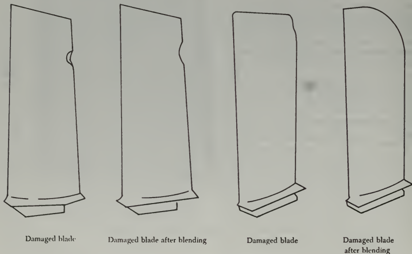
FIGURE 10-55. Compressor blade repair.
